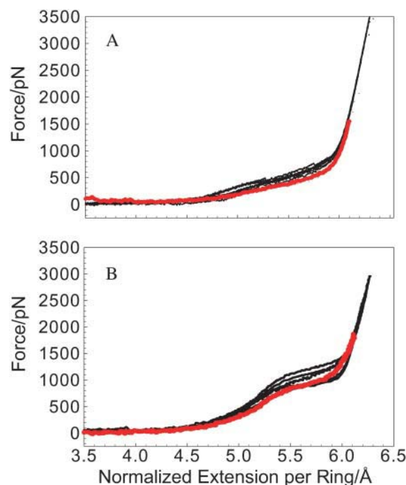
FIGURE 3 The elasticity of dextran and pustulan is not affected by solvents. We compare the experimental force-extension curves for pustulan (A) and dextran (B) obtained in water ( black traces ) and in solvents with a low dielectric constant ( \epsilon ) ( red traces ). (A) The red trace represents the force curve for pustulan obtained in dimethyl carbonate ( \epsilon = 3.1 ). (B) The red trace represents the force curve for dextran obtained in ethanol ( \epsilon = 25 ).
